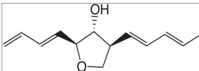
Aureonitol C 13 H 18 O 2 , 206.28 g/mol
